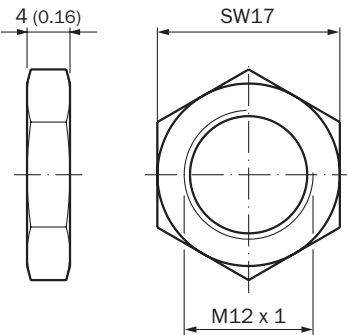
Dimensions in mm (inch)
