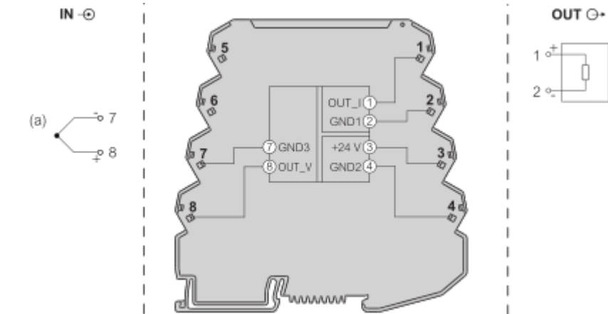
(a) : Thermocouple
