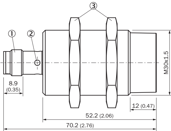
IMS30, V4A, non-flush
