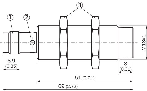
IMS18, V4A, non-flush
